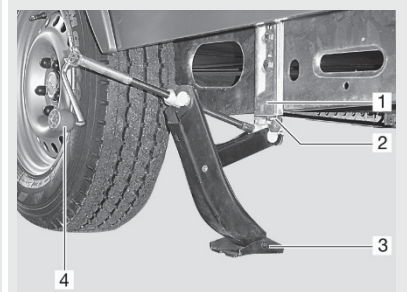
Fig. 224: Cric AL-KO
