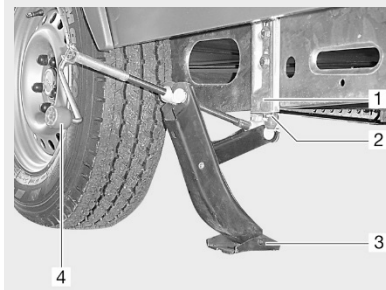
Fig. 160: Cric AL-KO
