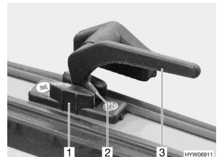
Afb. 99 Vergrendelingshendel in stand "continue ventilatie"
