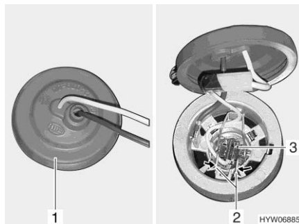
Afb. 220 Mistlamp
