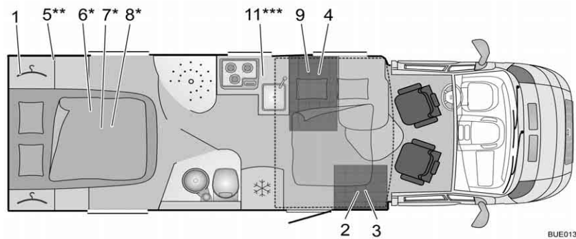
Fig. 302 Pianta IT 734 Ixeo Time
