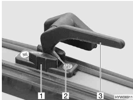
Afb. 69 Vergrendelingshendel in stand "continue ventilatie"
