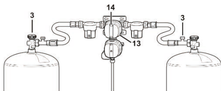
Fig. 109: Gasstrykkregulator-sett
