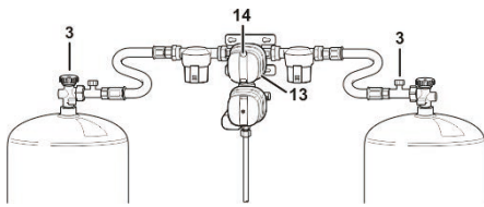
Fig. 106: Gasstrykkregulator-sett
