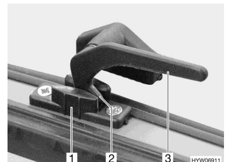
Afb. 72 Vergrendelingshendel in stand "continue ventilatie"
