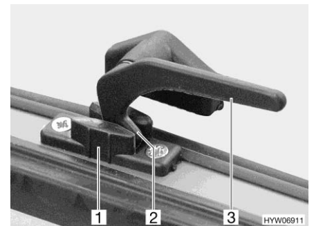
Afb. 114 Vergrendelingshendel in stand "continue ventilatie"
