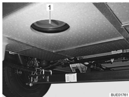
Afb. 211 Reinigingsopening afvalwatertank
