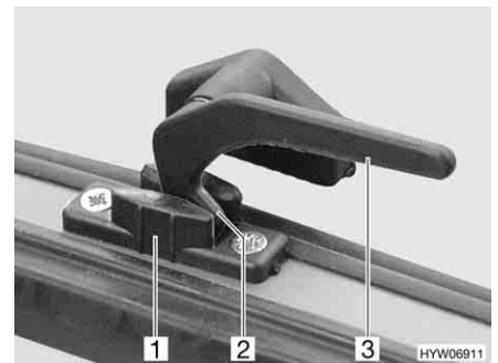
Afb. 60 Vergrendelingshendel in stand "continue ventilatie"
