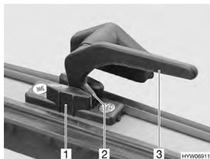
Afb. 65 Vergrendelingshendel in stand "continue ventilatie"
