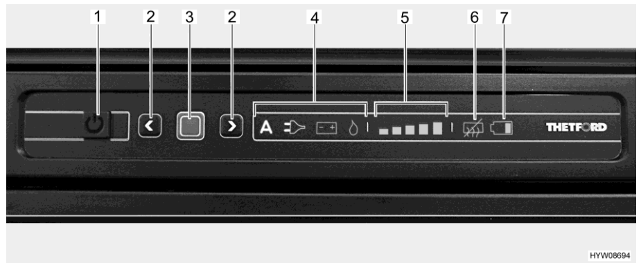
Afb. 242 LED-bedieningsveld (Thetford-koelkast)
