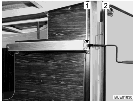
Afb. 131 Handslinger in garage achter
