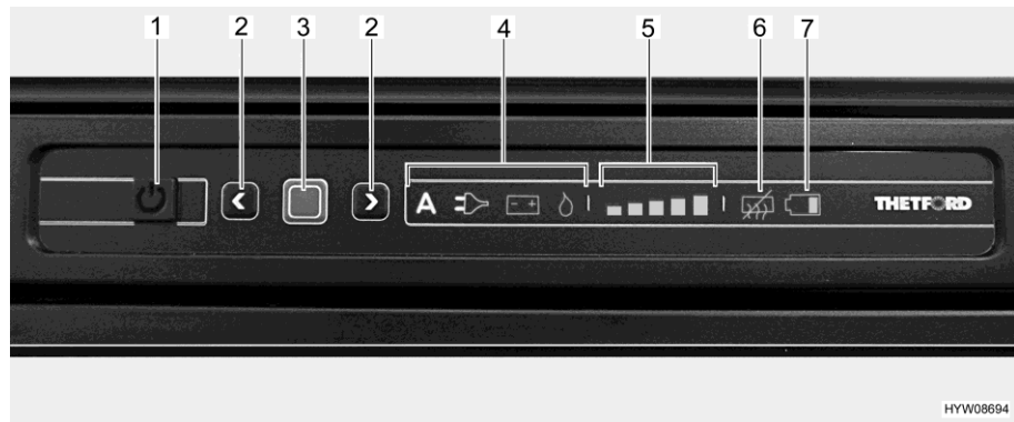
Afb. 249 LED-bedieningsveld (Thetford-koelkast)
