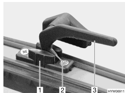
Afb. 117 Vergrendelingshendel in stand "continue ventilatie"
