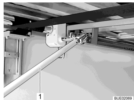
Afb. 133 Handslinger in garage achter
