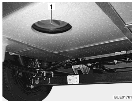
Afb. 291 Reinigingsopening (afvalwatertank)
