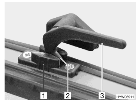
Afb. 94 Vergrendelingshendel in stand "continue ventilatie"
