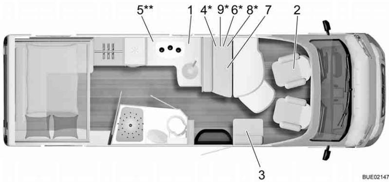
Fig. 289 Tracé Lyseo Harmony Line TD 744
