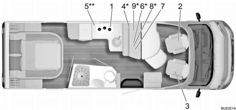
Fig. 290 Tracé Lyseo Harmony Line TD 745
