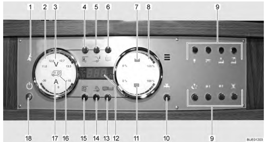
Fig. 107 Panel LT 510
