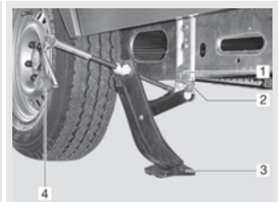
Fig. 150: Cric, AL-KO
