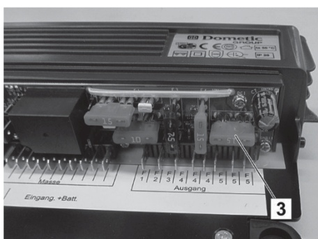
Fig. 57: 12 V Complete supply
