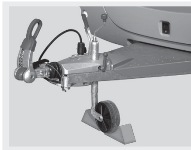
Fig. 139: Securing the support wheel
