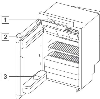
Fig. 132: Thetford Model A refrigerator
