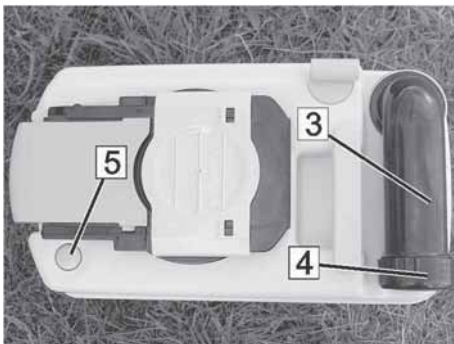
Fig. 124: Emptying the waste holding tank
