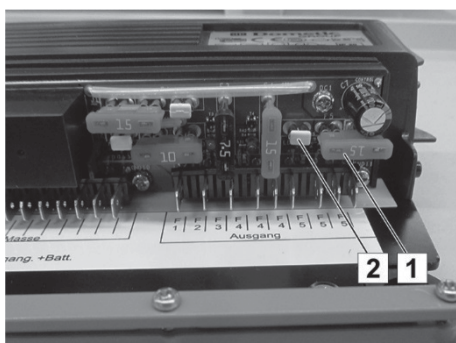
Fig. 56: 12 V Emergency lighting
