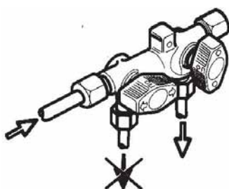
Fig. 71: Shut-off and release position
