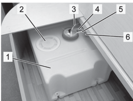
Fig. 77: Fresh water tank, example
