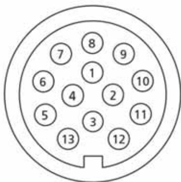
Fig. 2: 13-pole plug
